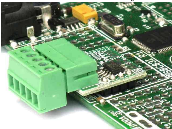
Picture 3: in485P Board inserted on target board
